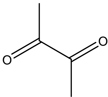
Biacetyl – model molecule
